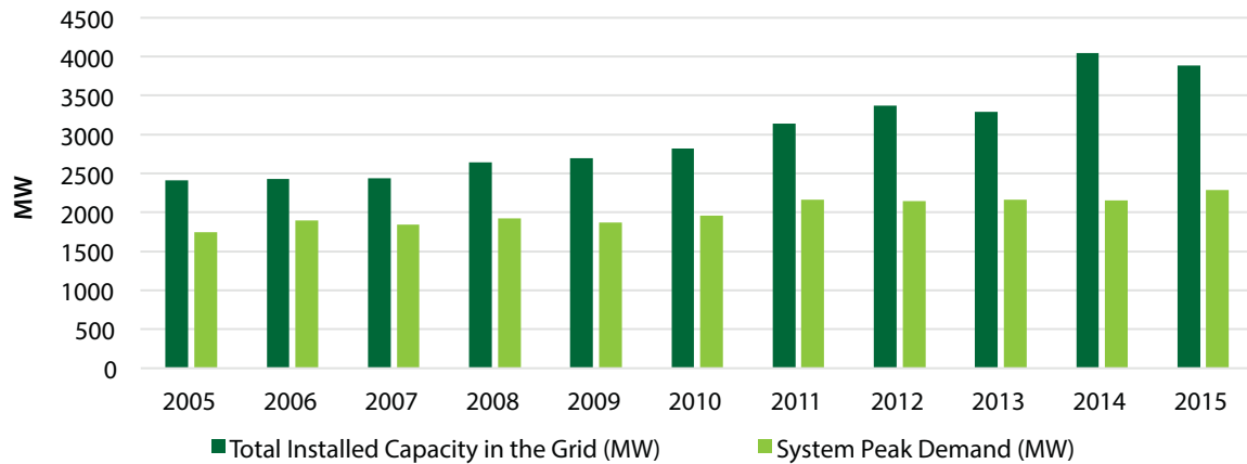
Figure 27: Trends in Electricity Supply and Peak Demand
