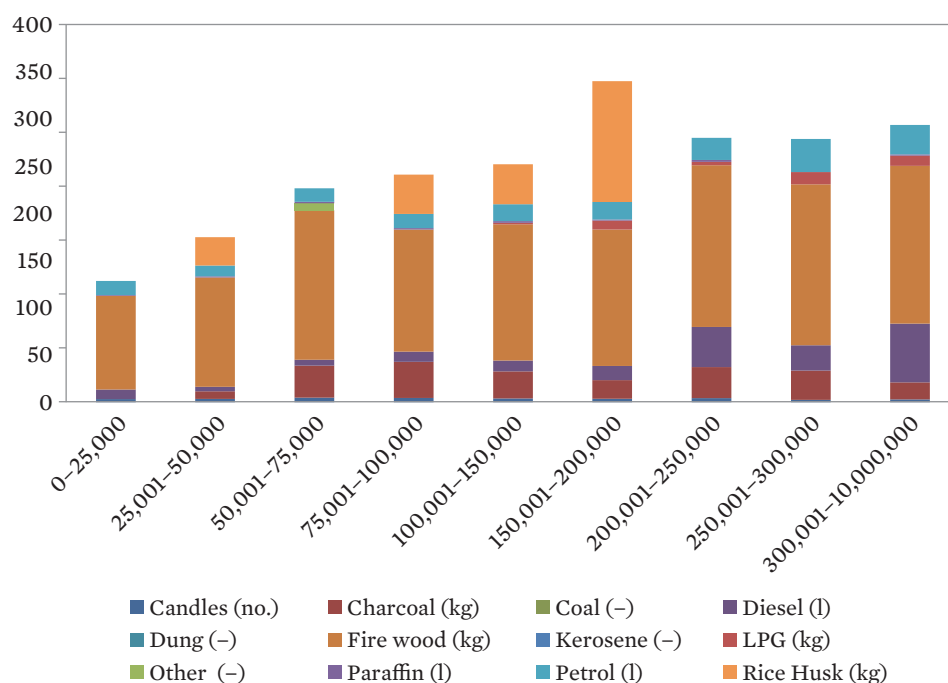
Figure 15: Quantity of Nonelectricity Fuel Being Used (All Townships)
