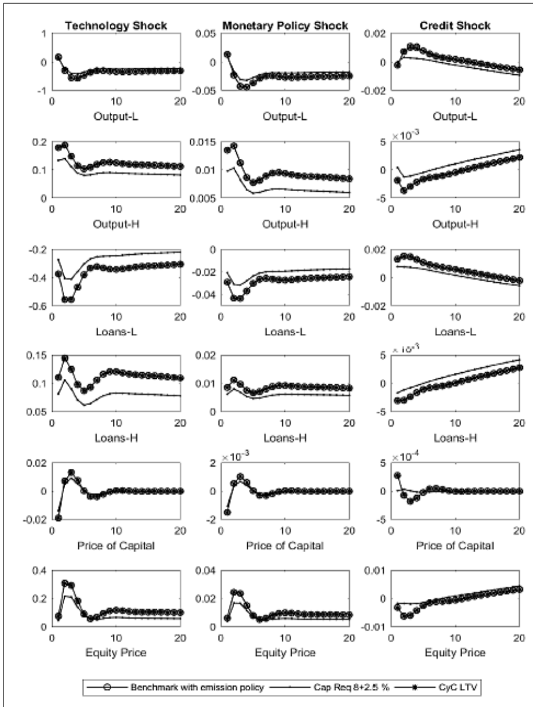
Figure 5: Policy Experiments
